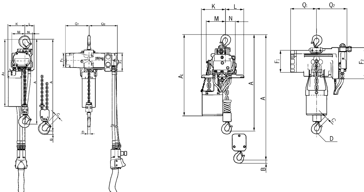
Model CPA ATEX 1-13 / 2-10 / 5-5
