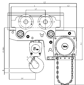
Model Yalelift LHP ATEX, 5000 kg, double fall
