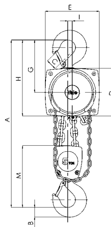
Model Yalelift 360 ATEX, 5000 kg, double fall
