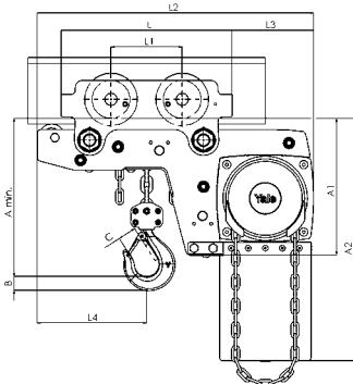
Model Yalelift LHG ATEX, 500 - 3000 kg, single fall
