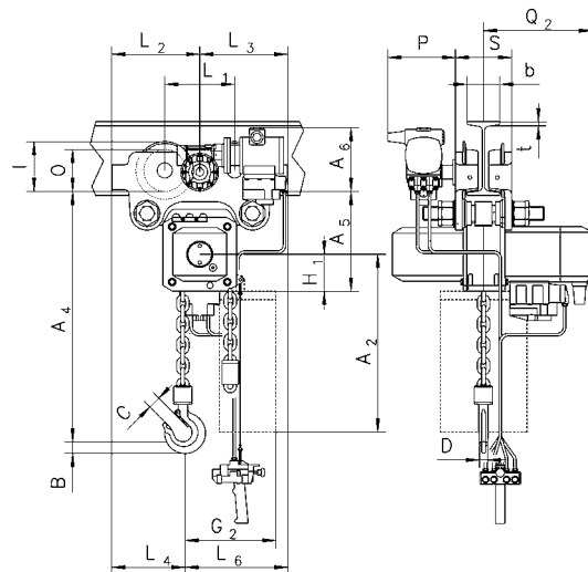
Model CPA ATEX with integrated pneumatic trolley
