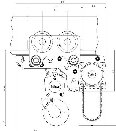
Model Yalelift LHG ATEX, 10000 kg, three fall
