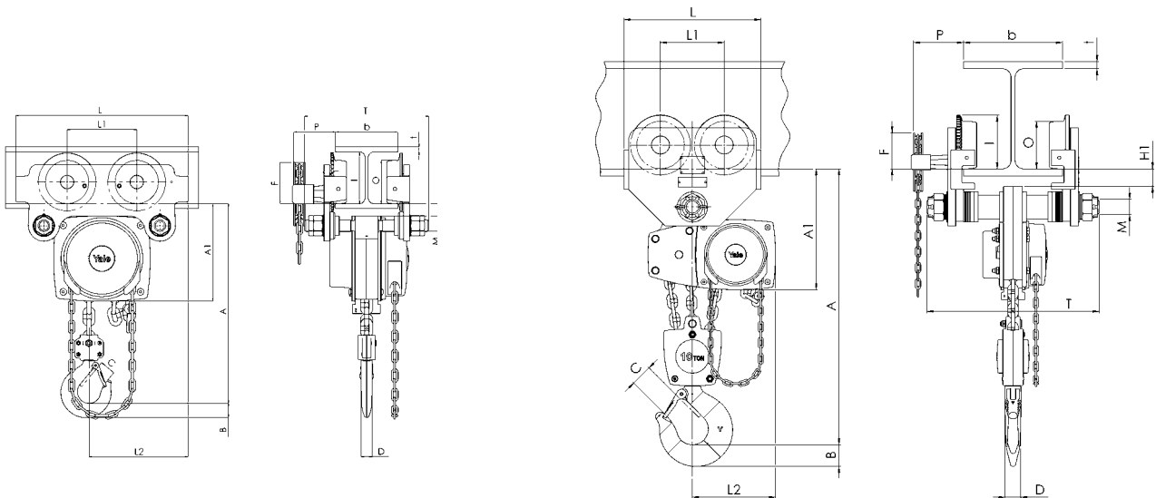
Model Yalelift ITG ATEX, 500 - 3000 kg, single fall
