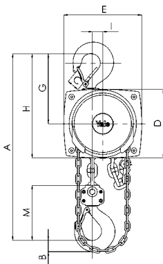
Model Yalelift 360 ATEX, 500 - 3000 kg, single fall
