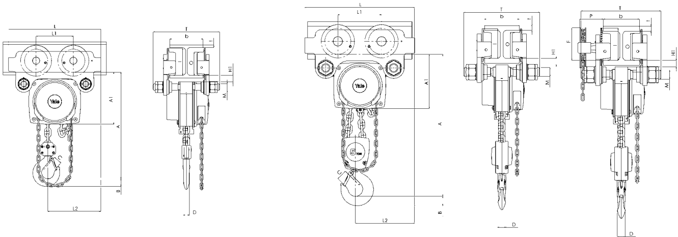
Model Yalelift ITP ATEX, 500 - 3000 kg, single fall
