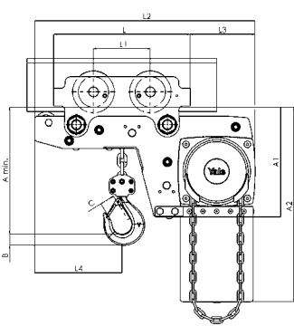
Model Yalelift LHP ATEX, 500 - 3000 kg, single fall
