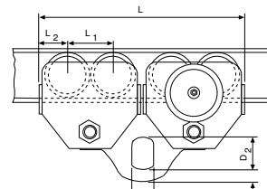
Model HTG ATEX, 20000 kg
